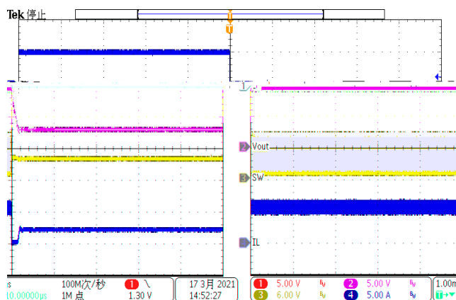
Figure 12. EN Power down (Iload=2A)
